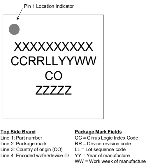
Figure 10-1. Package Marking
