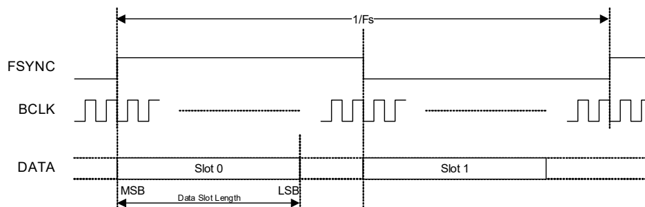
Figure 4-6. Left-Justified Data Format
