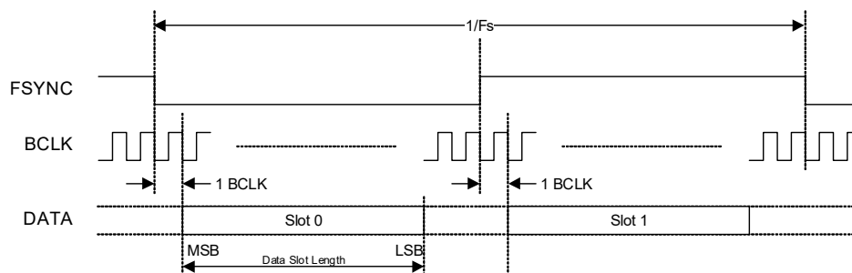
Figure 4-5. I 2 S Data Format
