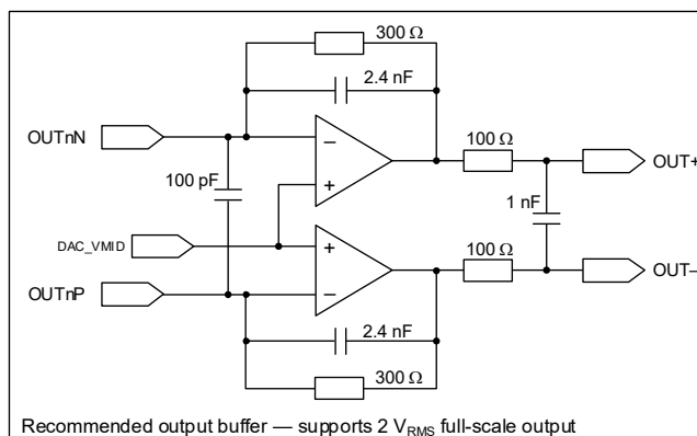
Figure 2-1. Typical Connections
