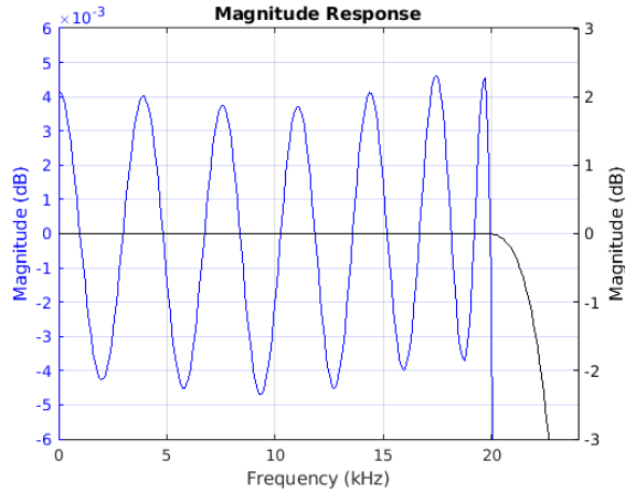
Figure 7-13. Passband Magnitude
